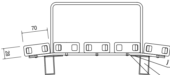
SECTION A~A' S=1/6
