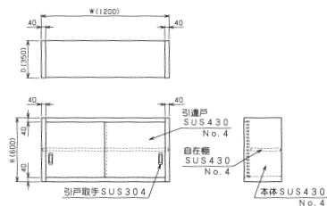
MCS6-1235SX
