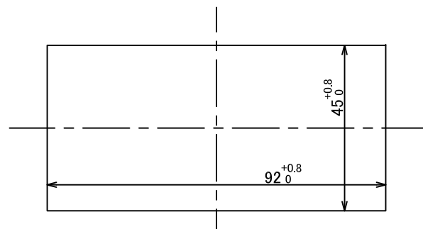
PANEL CUTOUT DIMENSIONS
