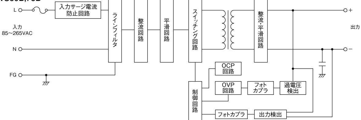
ZWS100B, 150B
