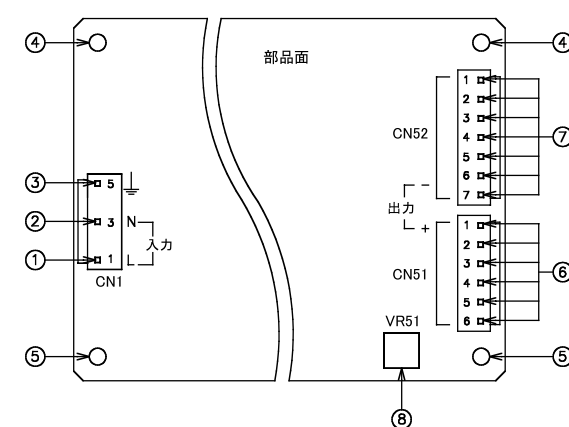
ZWS150B
