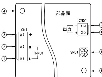
ZWS75B
