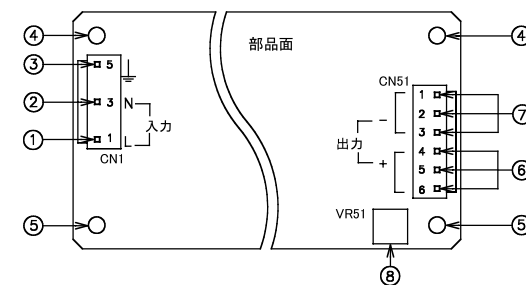
ZWS150B
