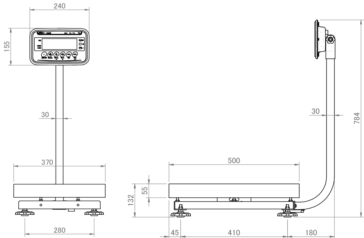
FG-60KCLWP FG-150KCLWP
