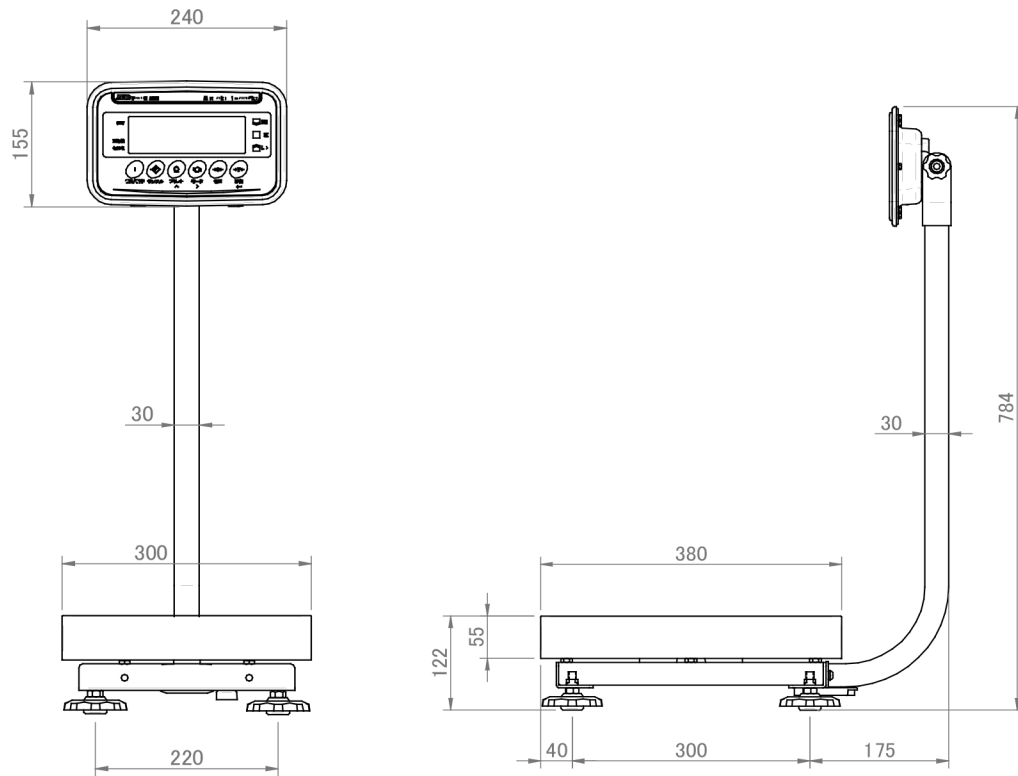
FG-60KCLWP FG-150KCLWP
