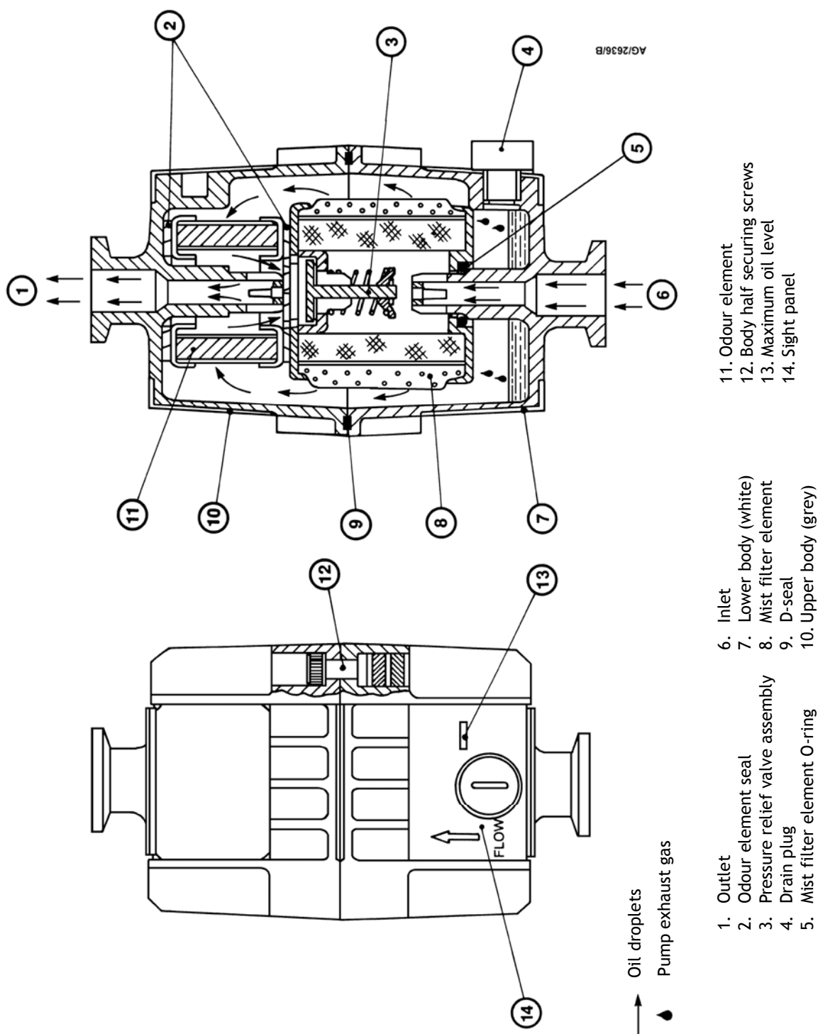
Figure 1 - Component parts of the EMF oil mist filters
