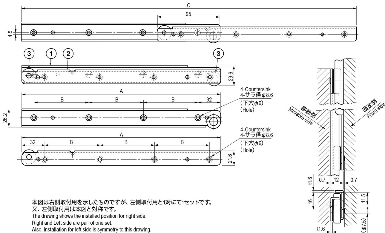
右側取付図 Installation Layout for Right Side
