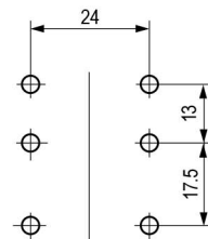
取付穴図 Holes for Installation
