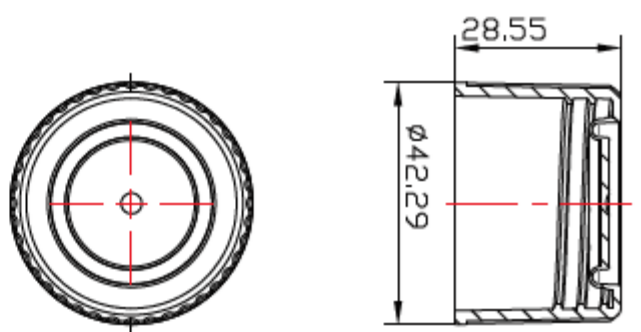
Plug Seal Cap
