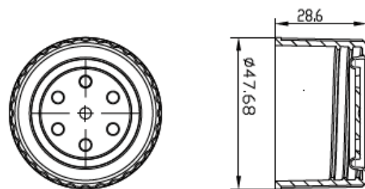
Plug Seal Cap
