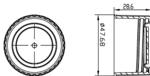
Plug Seal Cap
