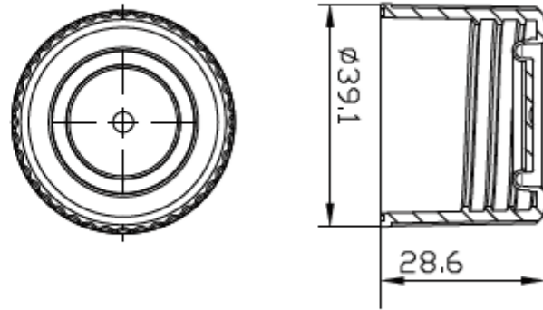
Plug Seal Cap
