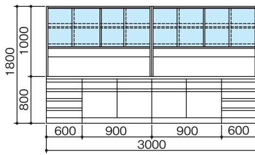
SQN-3075G
